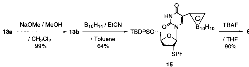
Scheme 3. Synthesis of 6
